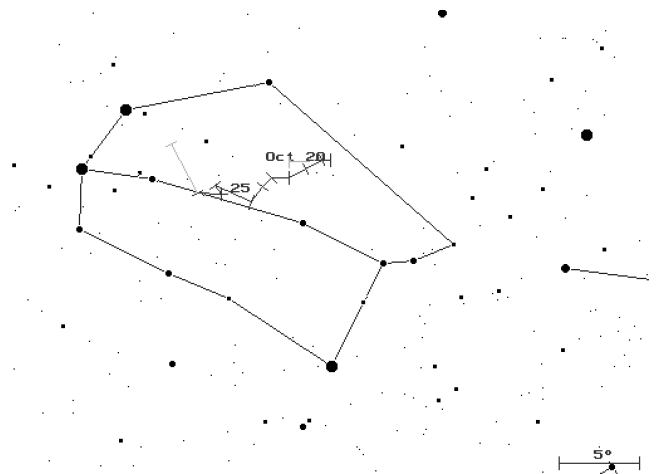
Figure 16 – Radiant of the \varepsilon -Geminids derived from the video data.
