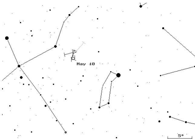
Figure 11 – Radiant of the \eta -Lyrids derived from our video data.
